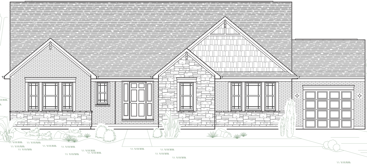
Elevation D 2058 sq. ft.
