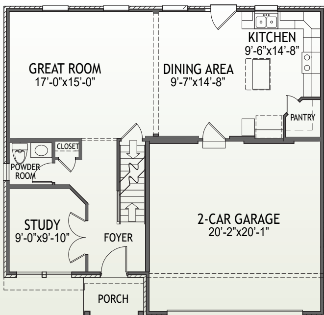
1st Floor
