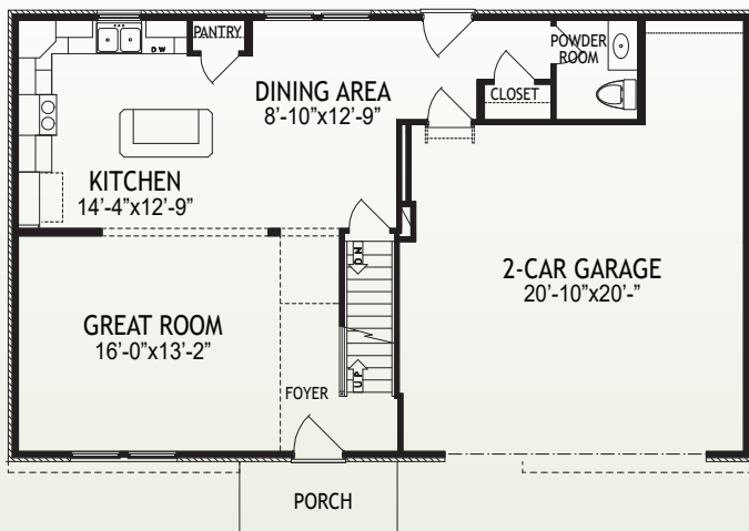
1st Floor
