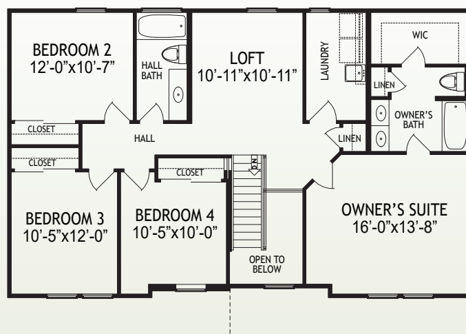
2nd Floor
