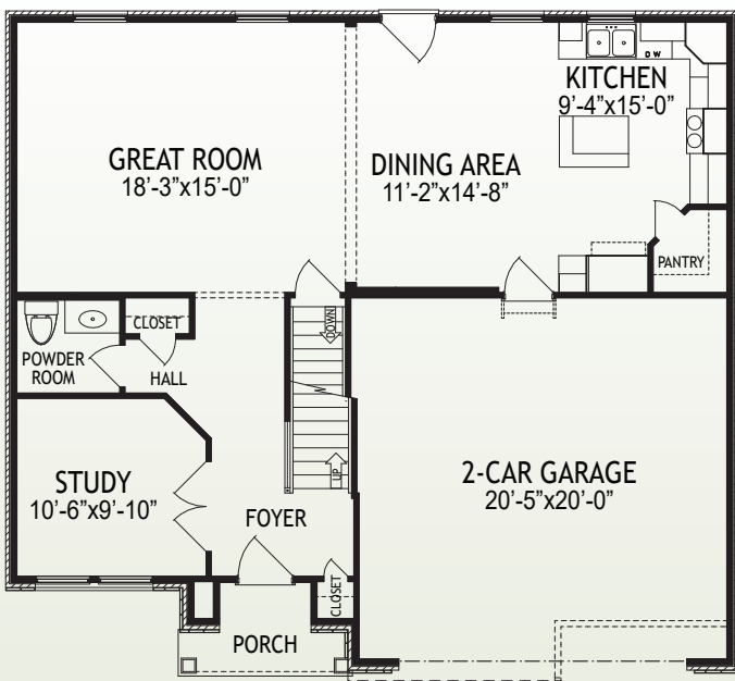
1st Floor
