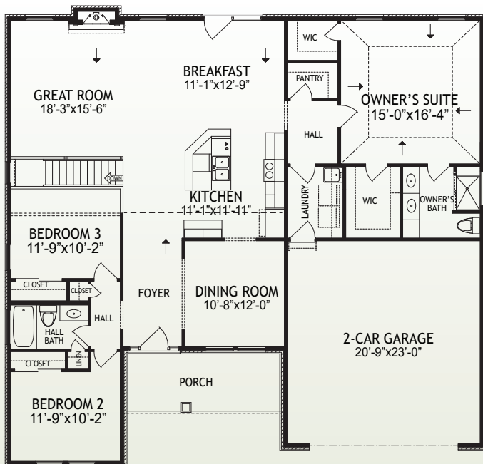
1st Floor
