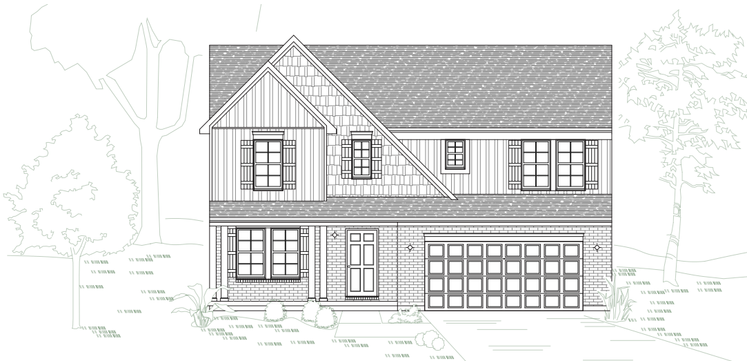
Elevation C 2285 sq. ft.
