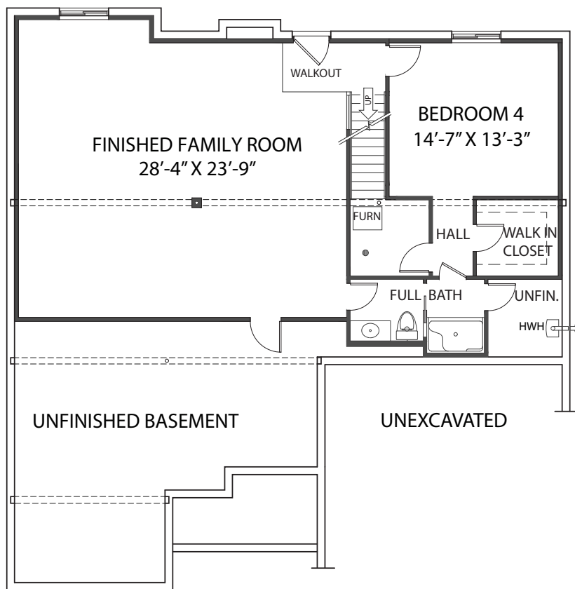
Optional Finished Lower Level
